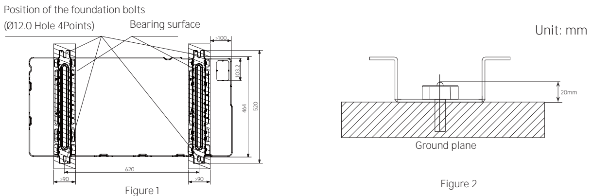
The base of the outdoor unit and the position of foundation bolts
